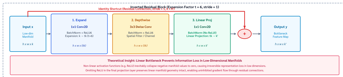
Panel (b): MobileNetV2 Inverted Residual Block with Linear Bottleneck (Micro-Architecture)
