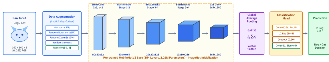
Panel (a): End-to-End Transfer Learning & Tensor Dataflow Pipeline (MobileNetV2 Backbone)
